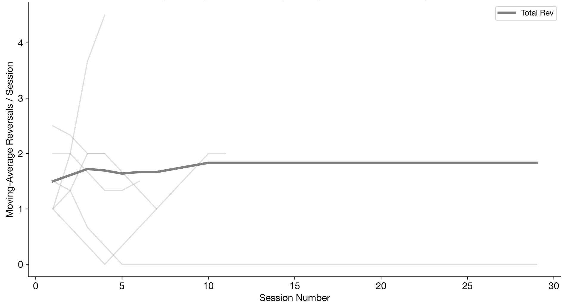
Moving-Average Total Reversals Over Time (n=6 subjects; sessions per subject=4–29; window=3)
